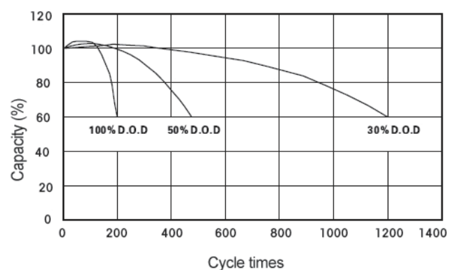
Cycle times and depth of discharge curve
