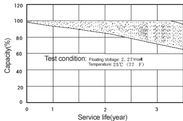
Floating charge service life characteristic curve - below 24Ah batteries
