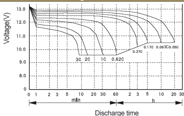
Discharge characteristic curve under different discharge rates (25°C)
