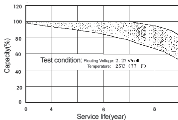
Floating charge service life characteristic curve - 24Ah and above batteries
