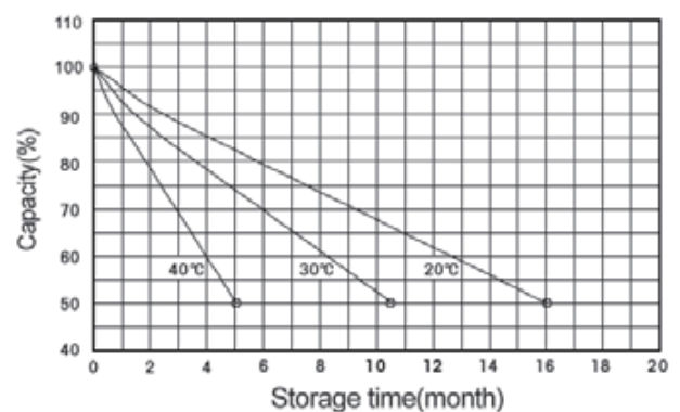
Discharge capacity and storage time curve
