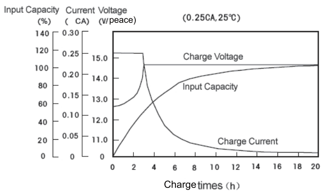
Charge characteristic curve
