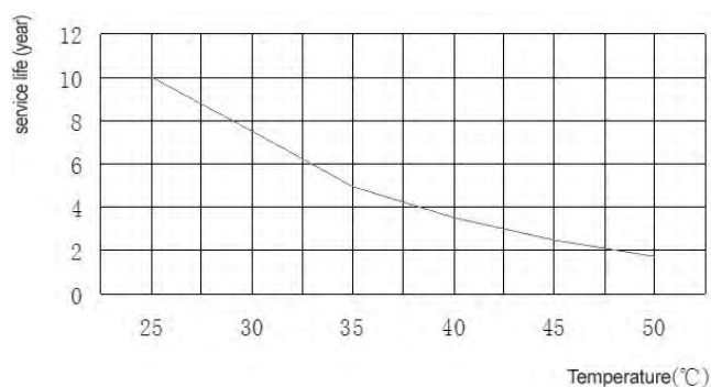
Service life and temperature curve SP series
