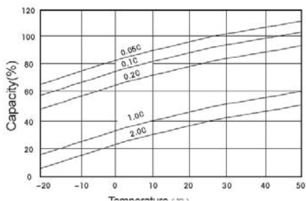
Discharge capacity and temperature curve
