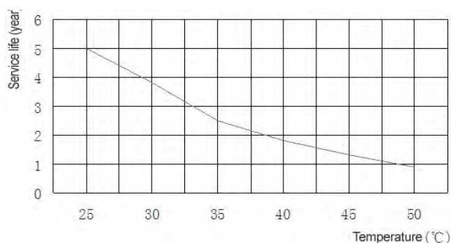
Service life and temperature curve SSP series
